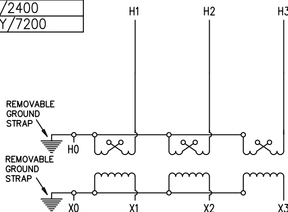
CONNECTION DIAGRAM
